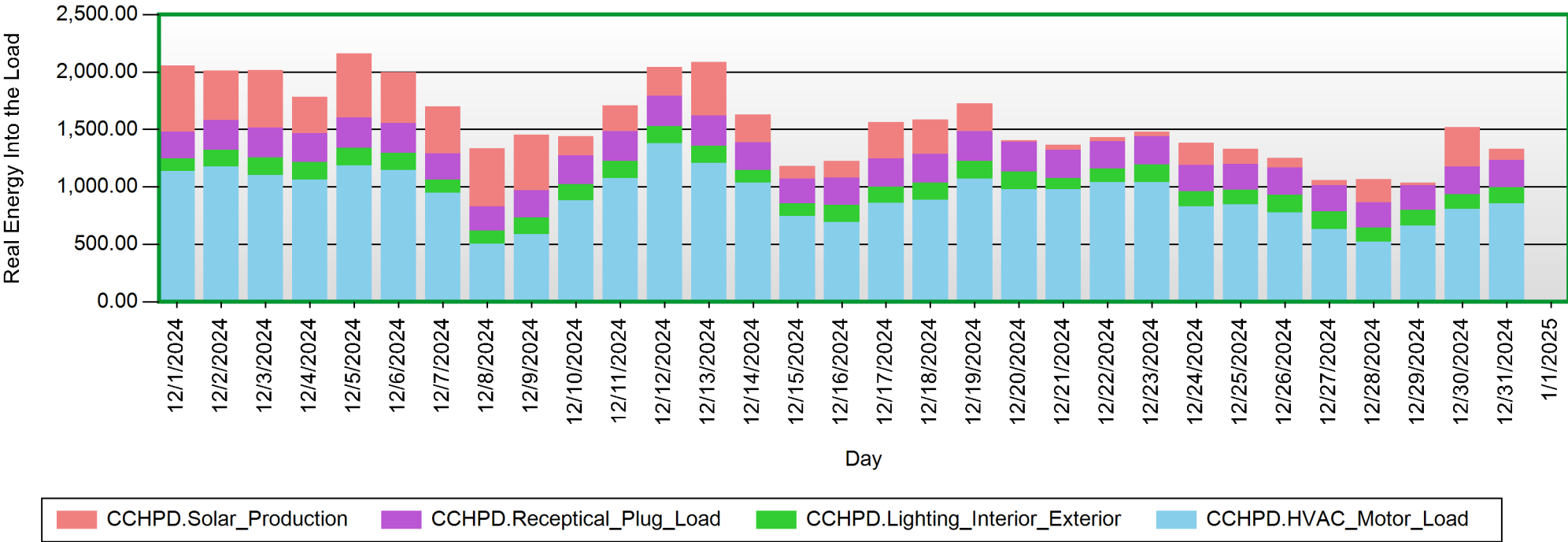
Energy Usage 00:00 - 00:00
